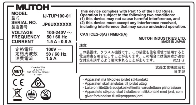
Rating plate
